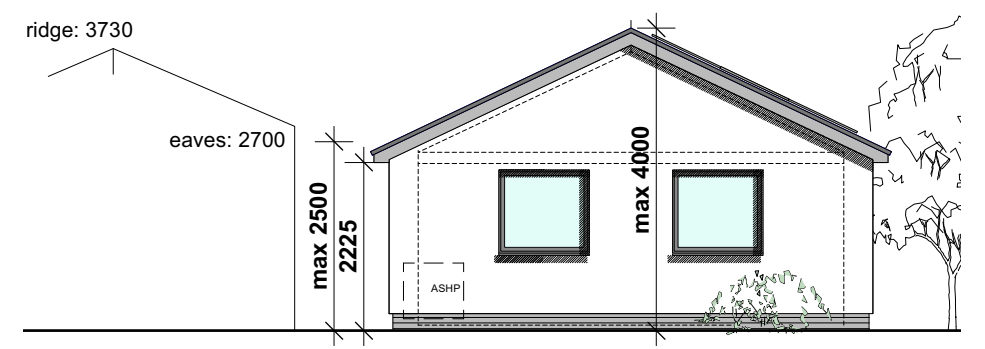
WEST ELEVATION
