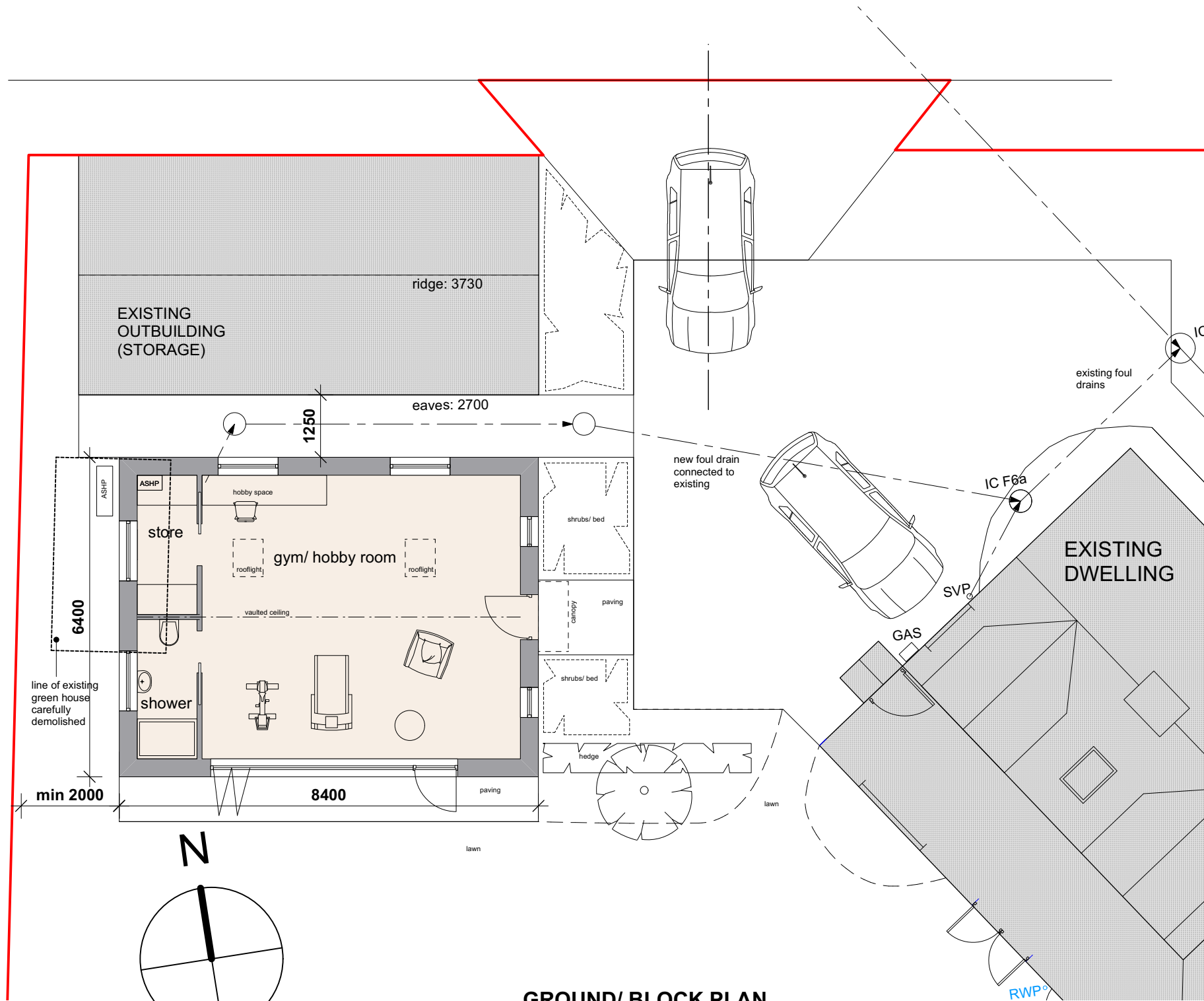
GROUND/ BLOCK PLAN
